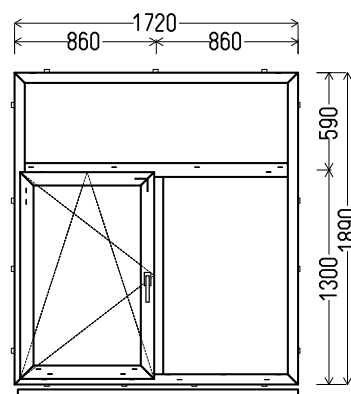
L3 (1vnt)
