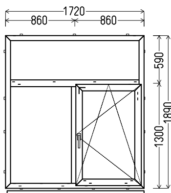
L1 (1vnt)
