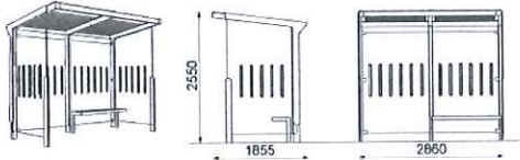
Bus stop shelter with flat roof steel structure, roof made of safety glass, rear and side walls made of tempered glass, without lighted advertisement box
