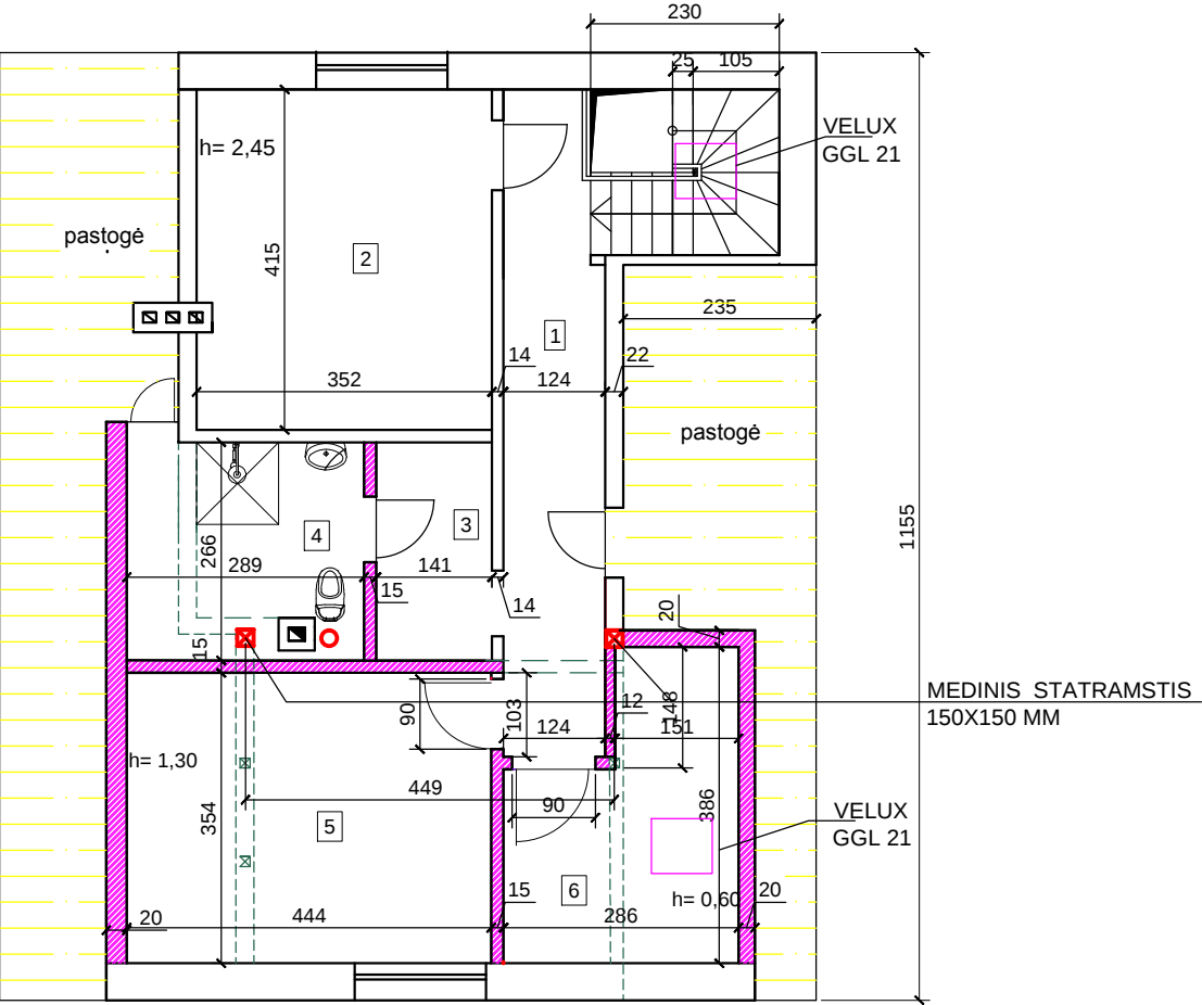
MANSARDOS PLANAS
