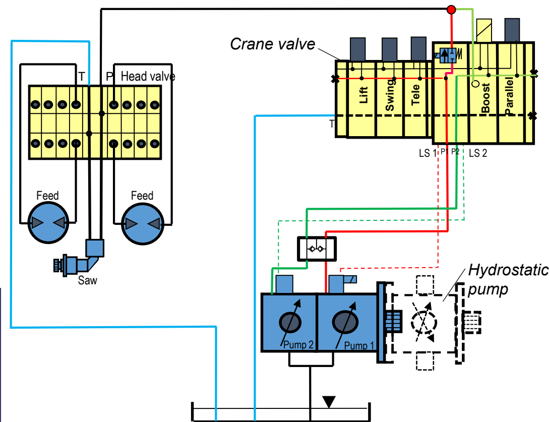
Circuit divisions schematic
