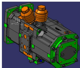
Dual pumps for working hydraulics
