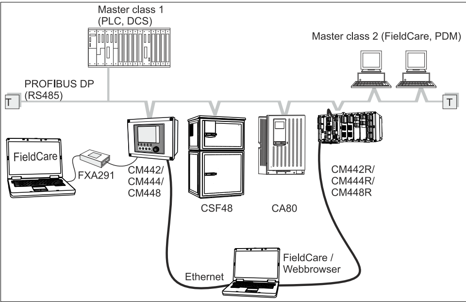
PROFIBUS DP T Terminating resistor
