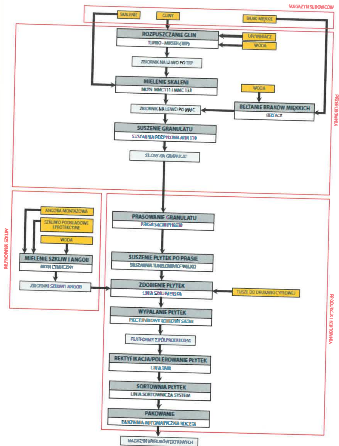
Fig. 1. The scheme of the production of the ceramic tiles with water absorption <0.5% by Cerrad Sp. z o.o.
