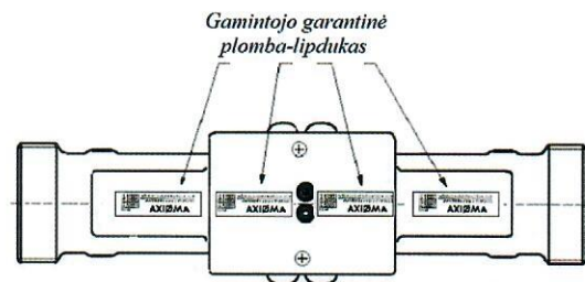
d) srauto jutiklio q_p = 10/15/25/40/60 \text{ m}^3/\text{h} plombavimas
