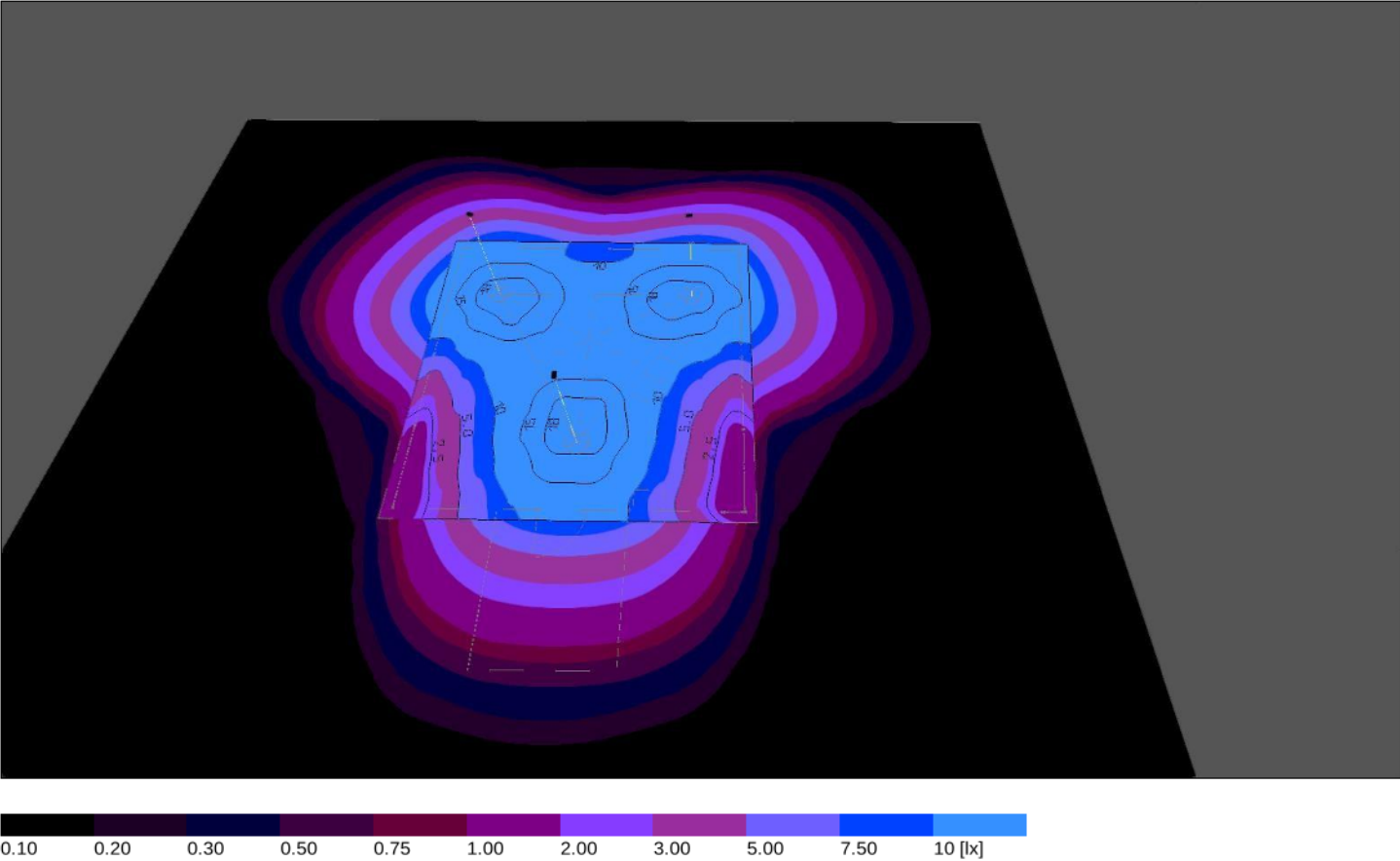
Site 1 (2), Illuminance values in [lx]
